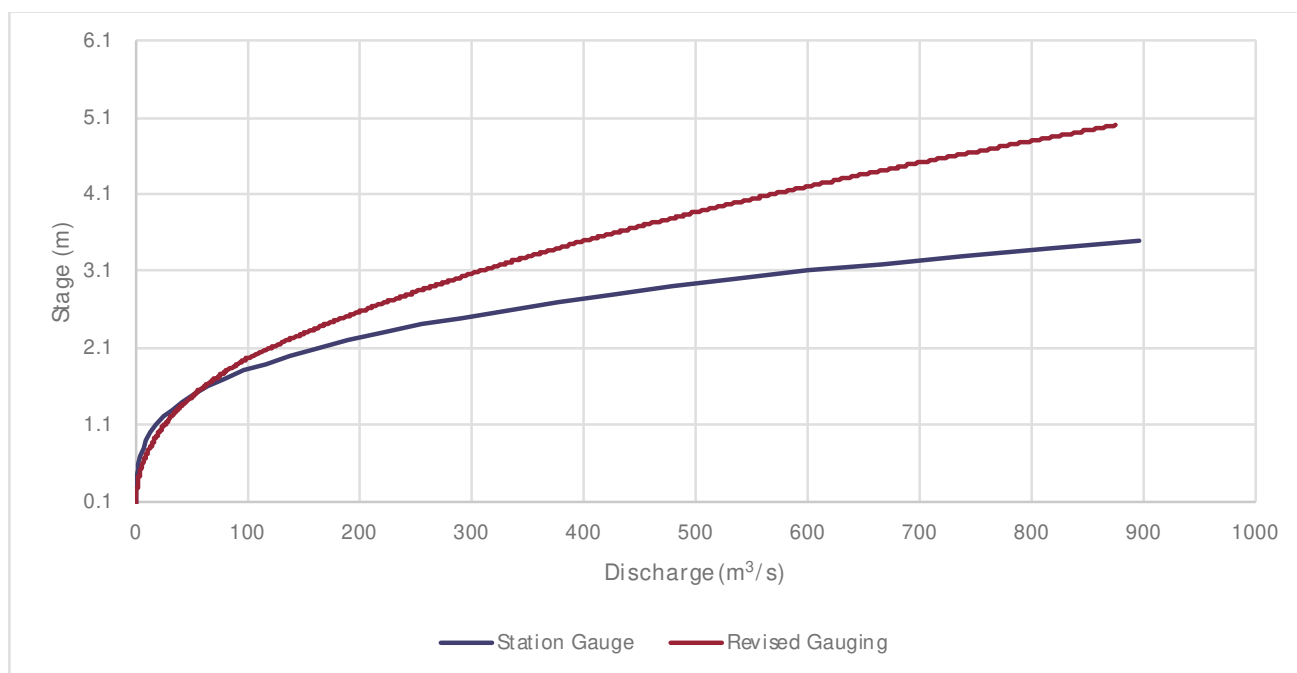
Figure B4 Rocky Hall Rating Curves
