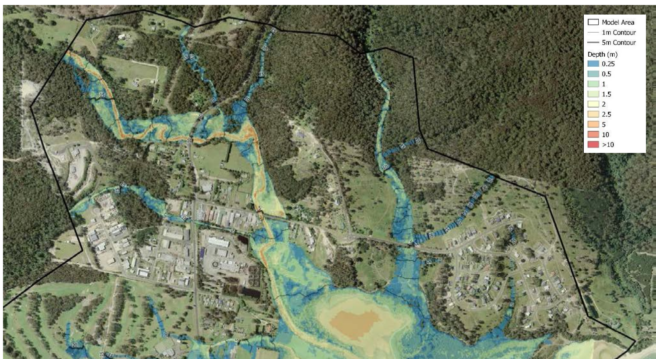
Figure 6-6 Lake Curralo Northern Tributaries (with 1% AEP flooding)
