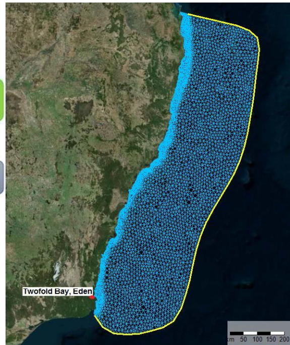
Figure 5-2 Method flow chart for Baird Australia's multihazard ECL Event Set (left) and the Delft3D NSW Tasman Sea Model Domain (right)
