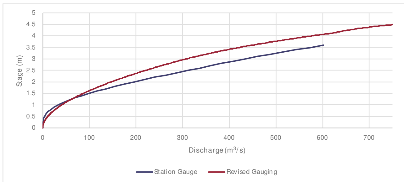
Figure B3 New Buildings Rating Curves
